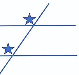
Corresponding Angles
