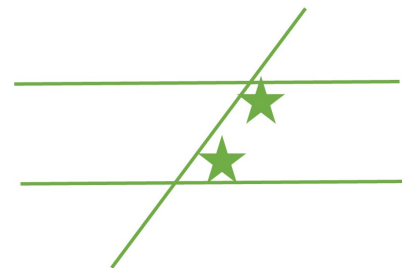
Co-interior Angles
