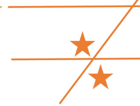
Vertical Angles
