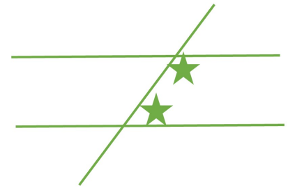
Co-interior Angles
