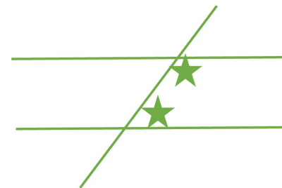
Co-interior Angles
