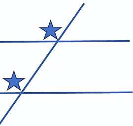
Corresponding Angles
