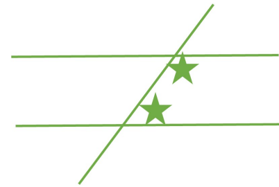
Co-interior Angles
