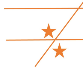
Vertical Angles
