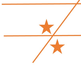
Vertical Angles
